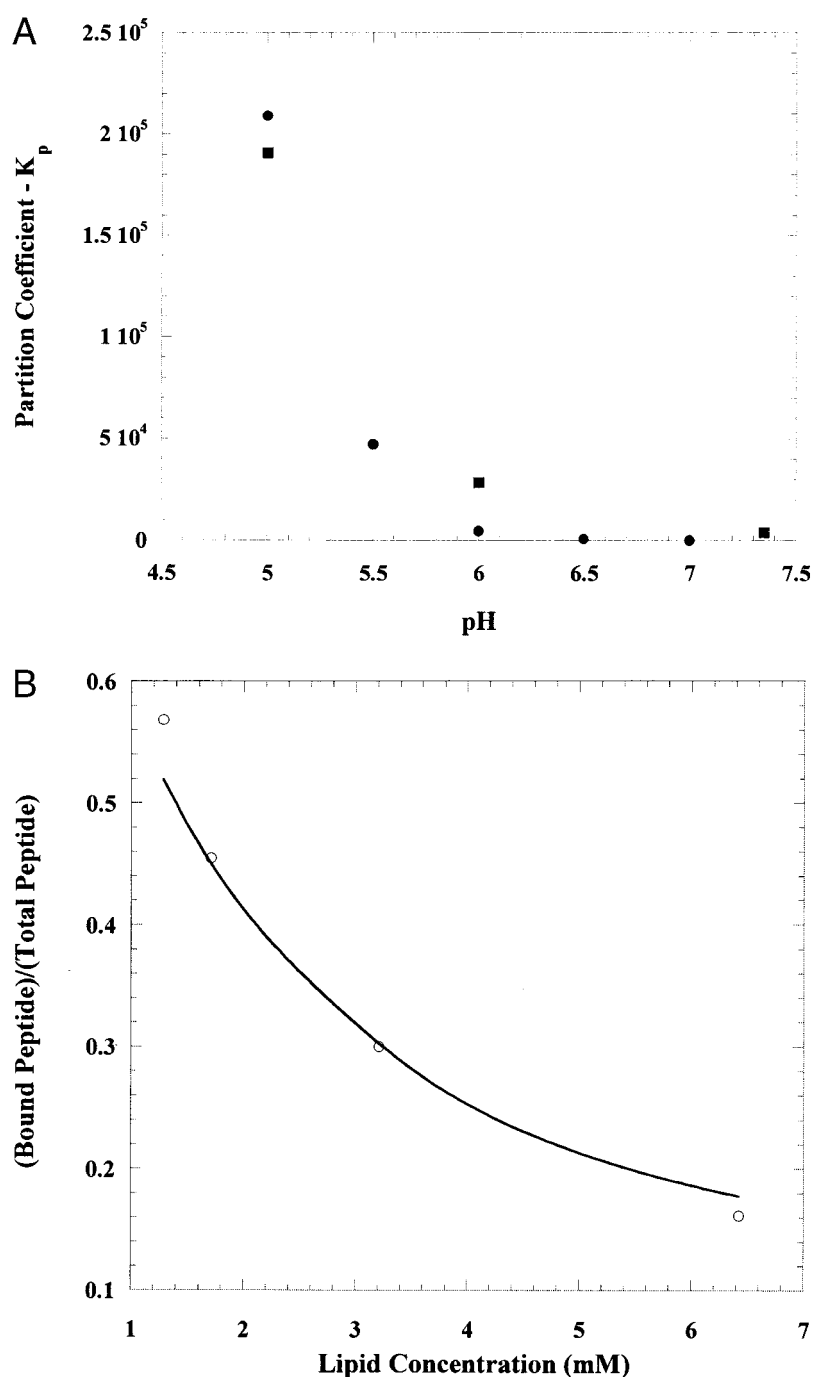
FIGURE 4 (A) Partition coefficient for SOPC membranes determined with the filtration method. The circles represent the data points for vesicles in phosphate buffer, and the squares are the data points for vesicles in the buffer used in the micropipette experiments (see Materials and Methods). The partition coefficient for pH 4.5, which is not shown in the graph, was 1 \times 10^6 . (B) Ratio of the bound peptide to the total peptide versus the lipid concentration, and the prediction of the model, assuming that all peptide in the solution was available for binding. The peptide concentration was 10 \mu\text{M} , and the pH was 5.5.
