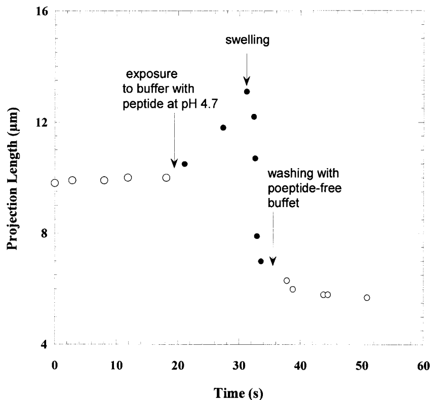
FIGURE 11 Reversible pores stimulated by AcE4K. The formation of pores was stimulated by exposing a single vesicle to peptide solution with reduced peptide concentration and with pH 4.7. After pore formation, the vesicle started to swell, and its projection length in the holding pipette started to decrease. During swelling, the vesicle was exposed to peptide free buffer with pH 4.7. The exposure to the peptide free buffer arrested the swelling of the vesicle and its projection length in the holding pipette approached a steady state. (The slow decrease of the projection length after the beginning of washing was due to peptide desorption).
