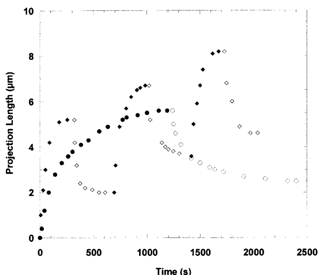
FIGURE 6 Peptide adsorption and desorption at pH 5.4. A single vesicle was exposed continuously to peptide buffer for 21 min (closed circles) and then the peptide was washed (open circles) with peptide-free buffer at the same pH. Another vesicle of similar size was exposed to peptide buffer (closed diamonds) and then washed (open diamonds) three times with peptide-free buffer. The total time of exposure of the two vesicles to peptide solution was the same. The projection length change after every washing of the adsorbed peptide was similar, and the final residual increase of the vesicle projection length was similar for the two vesicles. The change of the projection length during peptide desorption corresponded to 6% change of the vesicle area.
