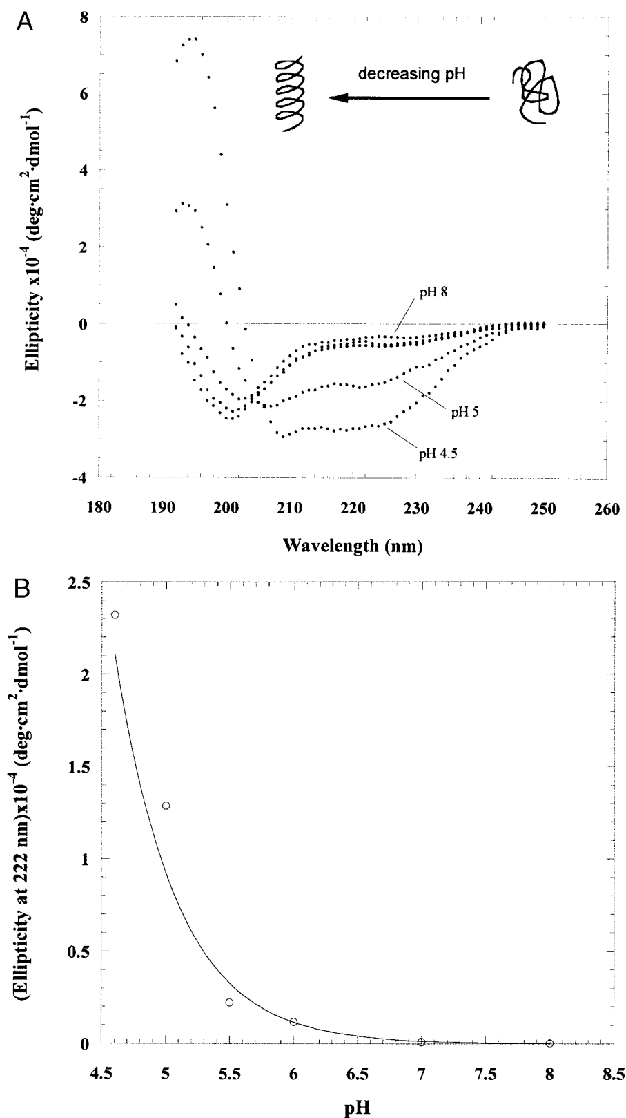
FIGURE 2 (A) CD spectra for AcE4K for lipid containing solutions with different pH. The peptide concentration was 10\ \mu\text{M} , and the lipid concentration was 0.36\ \text{mM} . The solid curve represents the calculated spectra for 100% ellipticity (see text). In the absence of lipid, the peptide remained in random coil conformation for the range of pH studied. In this case, the measured CD spectra (not shown) were almost identical to the CD spectra measured for lipid containing solutions at pH 8. (B) Change of AcE4K ellipticity at 222 nm versus pH.
