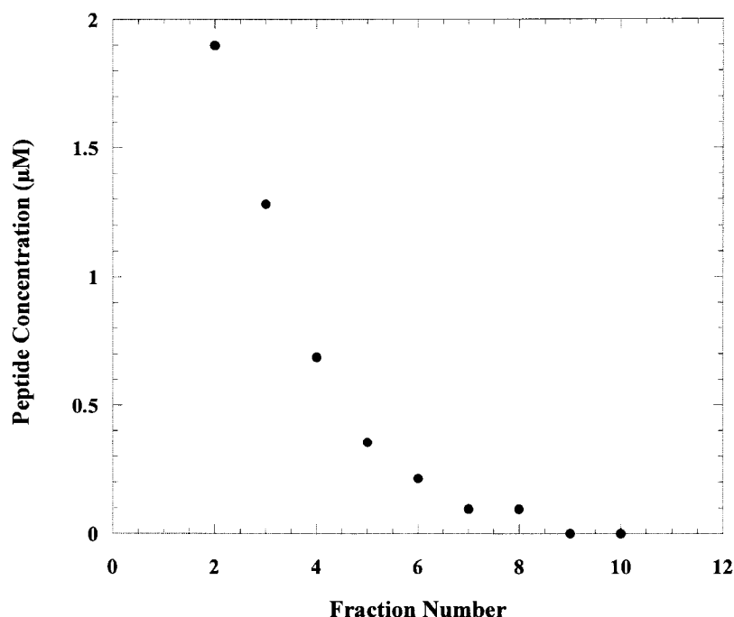
FIGURE 7 Peptide concentration of the sample fractions in the dilution experiment. The dilution for each fraction was 1:1. The peptide concentration in every following fraction was half of the concentration in the previous fraction. The initial peptide concentration in the sample was 10 \mu\text{M} , and the pH was 5.
