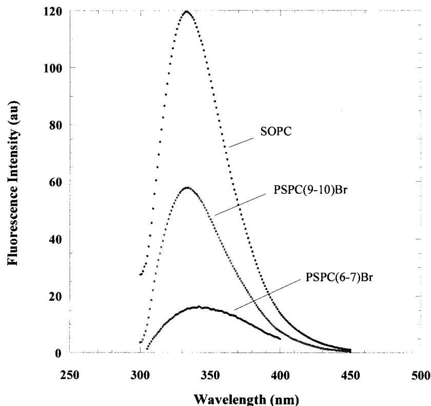
FIGURE 3 Fluorescence intensity of tryptophan from AcE4K inserted in SOPC membranes and membranes made of di-bromo lipids. The peptide concentration was 10 \mu M, and the pH was 5.
